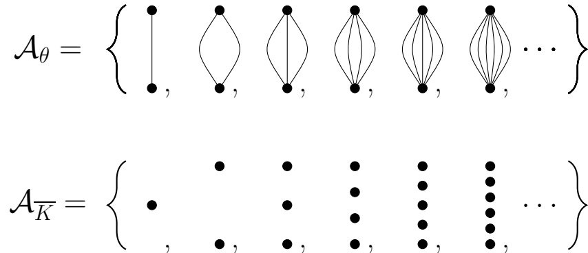
Figure 2: Two infinite antichains for contractions: multiedges and cocliques.
