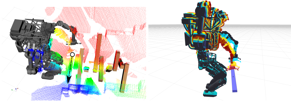
Figure 12: A fitting algorithm produces an affordance that can be used to plan a reach motion. Left: A line annotation (arrow) defines a search region that is used by a segmentation algorithm to fit a 2"x4" board affordance to the 3D point cloud data. Right: An end effector goal placed on the board affordance is used to compute a reaching plan.
