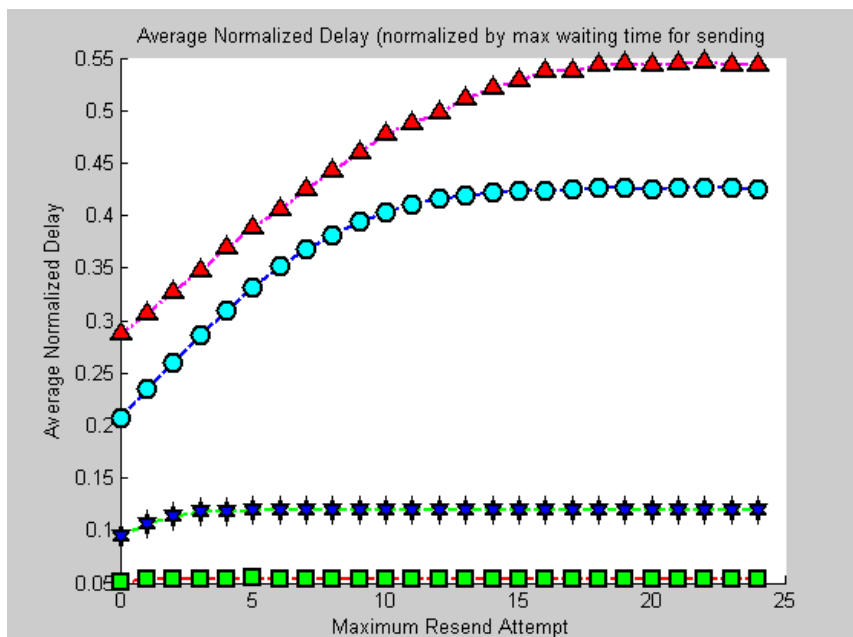
Figure 10: Average Normalized Delay versus maximum resend attempt (normalization with respect to the maximum waiting time for sending (24 slot—round trip slot))
