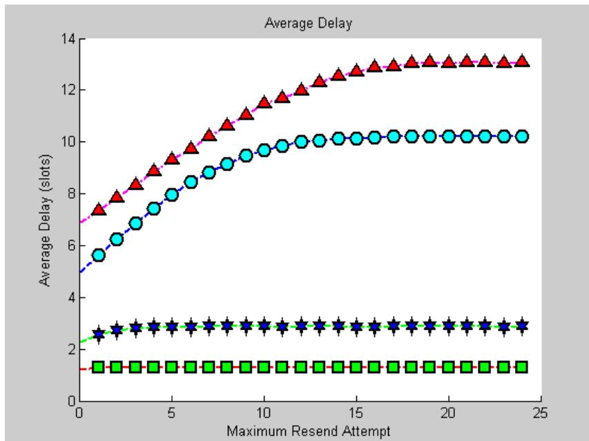
Figure 9: Average Delay versus maximum resend attempt.
