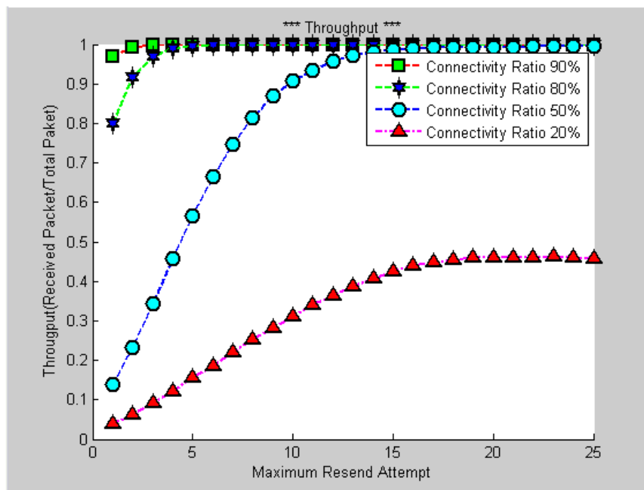
Figure 8: Throughput versus maximum resend attempt.
