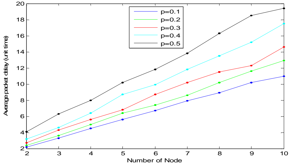
Figure 11: Delay Performance of Linear Topology ( p = P_{AN} = P_{NN} )
