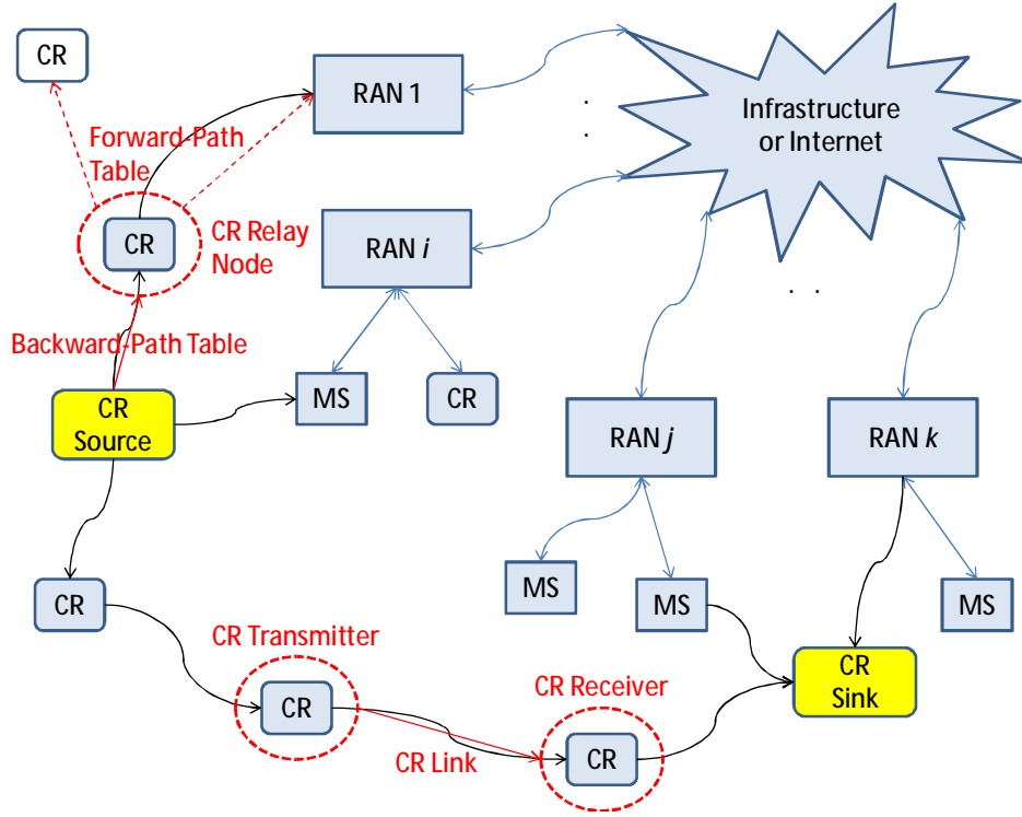
Figure 4: CLOD Routing
