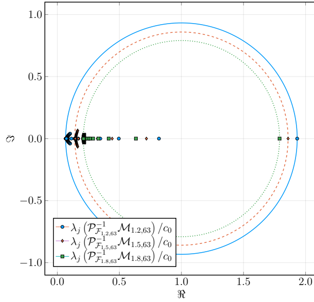
Figure 2: [Example 1: 1D, \alpha = \{1.2, 1.5, 1.8\} ] Scaled spectra of the resulting matrices when the preconditioners \mathcal{P}_{\mathcal{F},n_1} are applied to the coefficient matrices \mathcal{M}_{\alpha,n_1} for n_1 = 2^6 - 1 .
