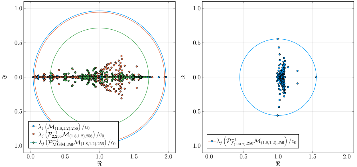
Figure 6: [Example 3: 2D, \alpha = 1.8, \beta = 1.2 ] Scaled spectra of the resulting matrices when the preconditioners are applied to the coefficient matrices \mathcal{M}_{(\alpha,\beta),n_1^2} and n_1 = 2^4 . Left: Preconditioners \mathbb{I}_N , \mathcal{P}_{2,N} , and \mathcal{P}_{\text{MGM},N} Right: Preconditioner \mathcal{P}_{\mathcal{F}(\alpha,\beta),N} .
