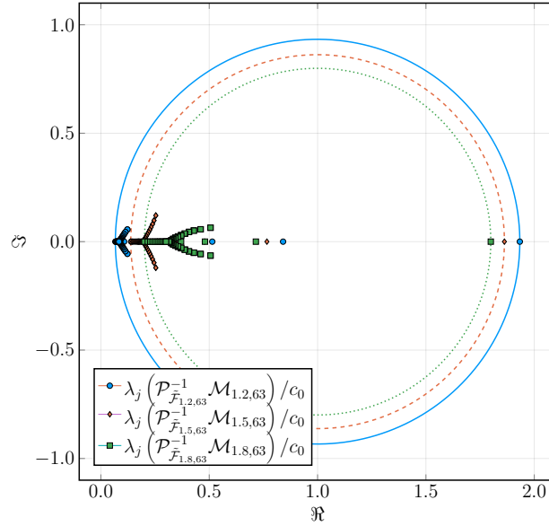
Figure 4: [Example 1: 1D, \alpha = \{1.2, 1.5, 1.8\} ] Scaled spectra of the resulting matrices when the preconditioners \mathcal{P}_{\tilde{\mathcal{F}},n_1} are applied to the matrices \mathcal{M}_{\alpha,n_1} for n_1 = 2^6 - 1 .
