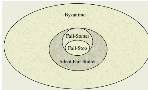
Fig. 1. Different fault models and their relation
