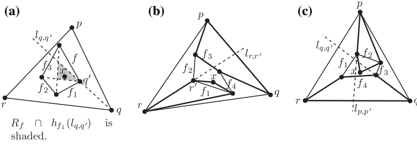
Fig. 10. |H| = 3 , |H'| = 4
