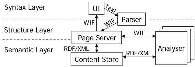
Fig. 1: Architecture of a Semantic wiki
