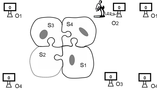
Fig.3: A hypothetical perspective of O_2
