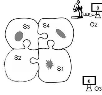
Fig.4: The real perspective of O_2
