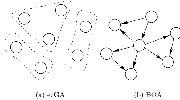
Fig. 1. Representation of the models used in the ecGA and the BOA.
