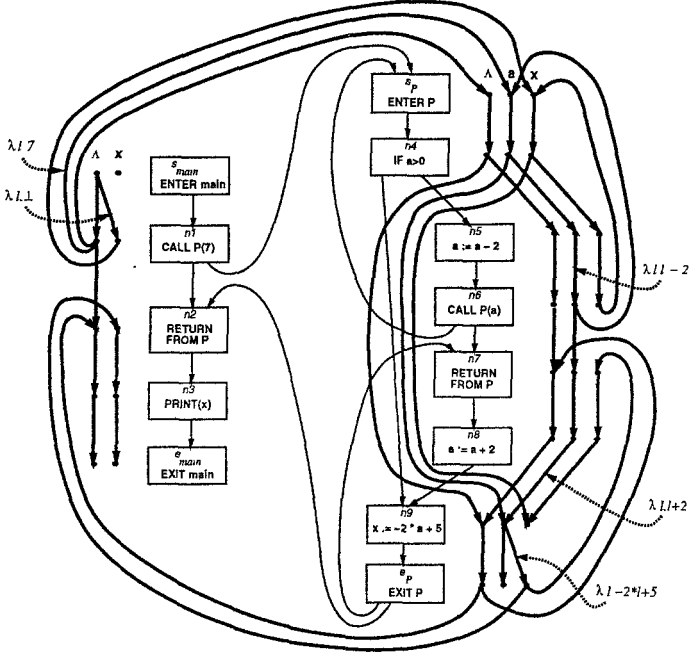
FIGURE 2. The labeled exploded supergraph for the running example program for the linear constant-propagation problem. The edge functions are all \lambda l.l except where indicated.
