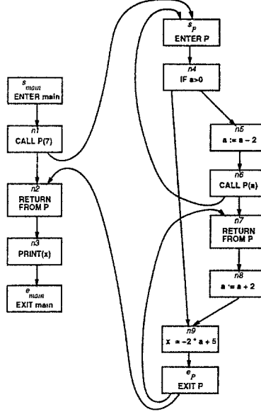
FIGURE 1. An example program and its supergraph G^* .
