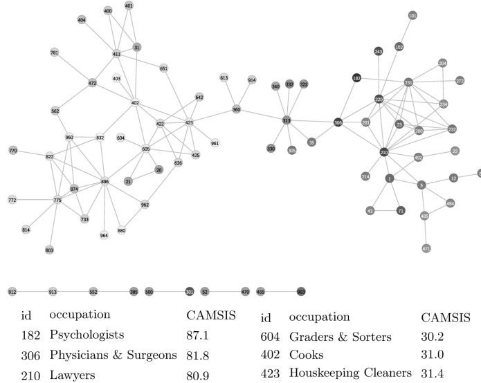
Fig. 5. Network of occupations derived from US census data of 2000. Node color indicates the CAMSIS scores of occupations. The darker the node, the higher the score. The table shows the three occupations with the highest (left) and lowest (right) CAMSIS scores.
