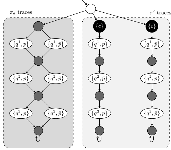
Fig. 5: Kripke structure for the formula y = \exists x_1. \forall x_2. \exists x_3. (x_1 \vee \neg x_2 \vee x_3) \wedge (\neg x_1 \vee x_2 \vee \neg x_3) .
