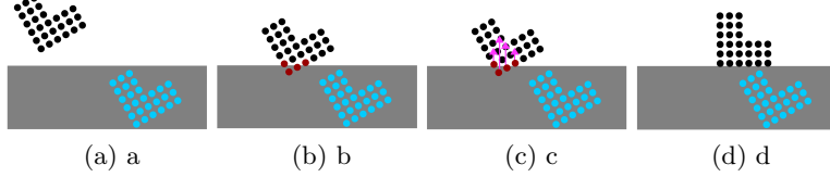
Fig. 6. The collision resolution process used by our lightweight simulator. From left to right, (a) a robot represented by points (black) moving towards a target (light blue) and an obstacle (gray) (b) collides with the object, triggering the collision resolution. (c) point corrections \Delta p_n for each colliding point of the robot are computed from the surface normals of the object and applied (d) so the robot complies to produce an in-contact state.
