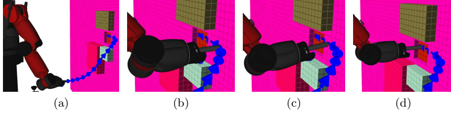
Fig. 4. An execution of the Baxter task, from start (a) to goal (d), and environment with confined space around the goal. The planned policy is shown in blue. Note the use of contact with the environment to reduce uncertainty and reach the target passage.
