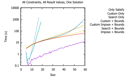
Fig. 3: Comparing baseline solutions with different search strategies
