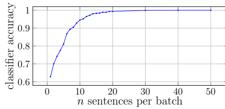
Fig. 2: Accuracy of the classifier in different setting of n .
