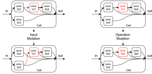
Fig. 4: Mutation operations available in randomized evolution. When input operation is applied, previous input block is linked with cell output if it has remained pendent, avoiding block removal.
