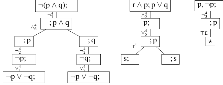
Figure 1: Examples of derivations in tree form. For the sake of a cleaner presentation, we omit the formulas that are inherited when expanding a node.
