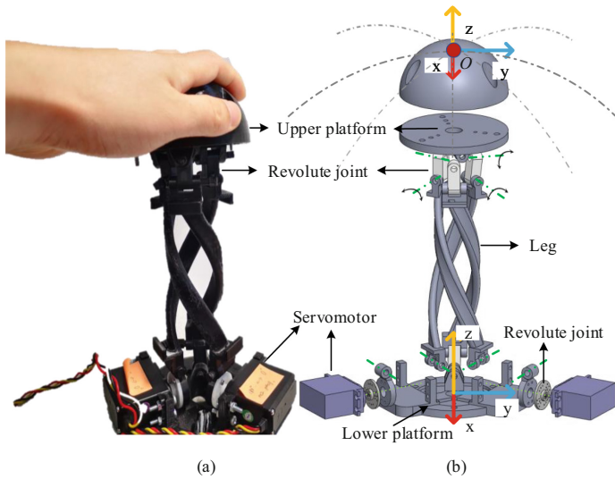
Fig. 1. The device is composed of two servo motors actuating an anti-parallelagram mechanism moving two platforms with respect to each other. (a) Device in its grounded configuration, with the lower platform secured to an external support and the user hand posed on the upper one. The device can be either used as a grounded interface, like in this figure and in our experiment of Sect. 3, or it can be held between the two hands (see the video for this configuration). (b) CAD of the device. The grey dotted lines show the surface of the sphere on which the upper platform moves. The spherical cap posed on the upper platform makes the interaction with the user hand more comfortable. Of course, it can be changed with other shapes according to the task at hand. (Color figure online)
