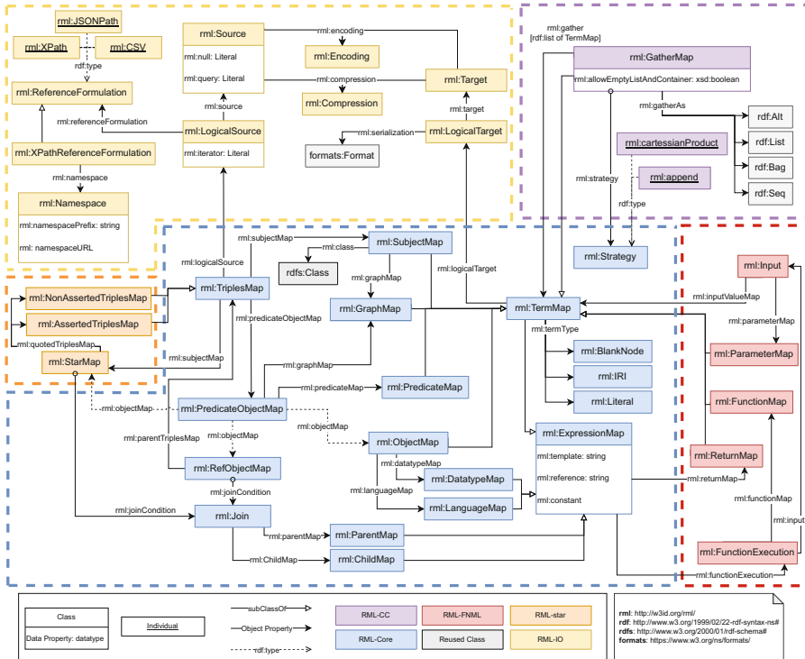
Fig. 1. RML ontology overview following the Chowlk diagram notation [34].
