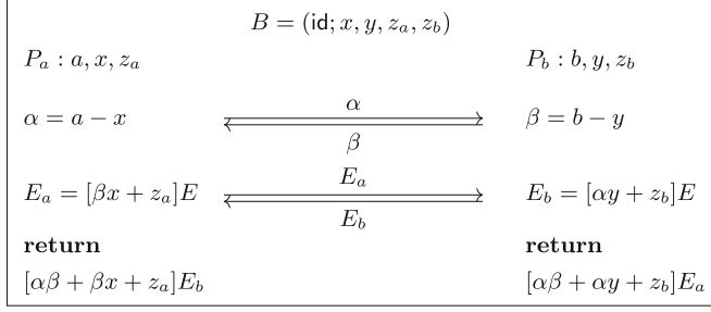
Fig. 2. Passively secure 2-party multiplication protocol from additive secret sharing, using a trusted tuple B as input.
