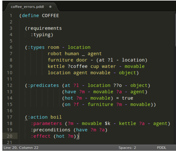
Figure 1: Syntax highlighting using MYPDDL-IDE. White text contains errors.
