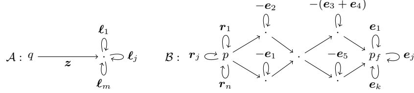
Fig. 1. Illustration of the approach to reduce validity of a \Pi_2 -PA formula \Phi = \forall \mathbf{x}. \exists \mathbf{y}. (t_1 \vee t_2) \wedge ((t_3 \wedge t_4) \vee v_5) to inclusion for \mathbb{Z} -VASS.
