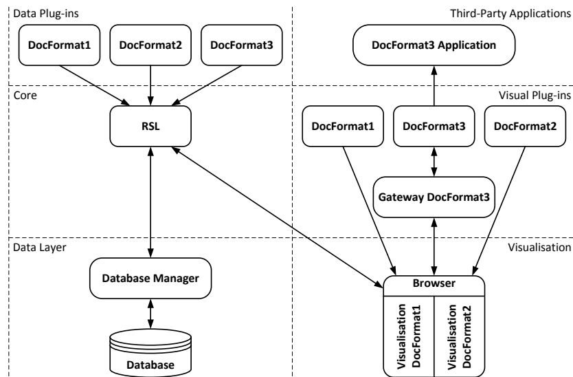
Fig. 1: General open cross-document link service architecture
