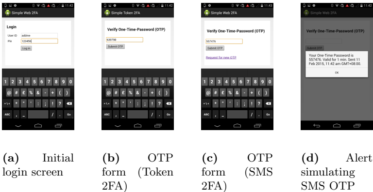
Fig. 3. Web application components for the Token and SMS investigations
