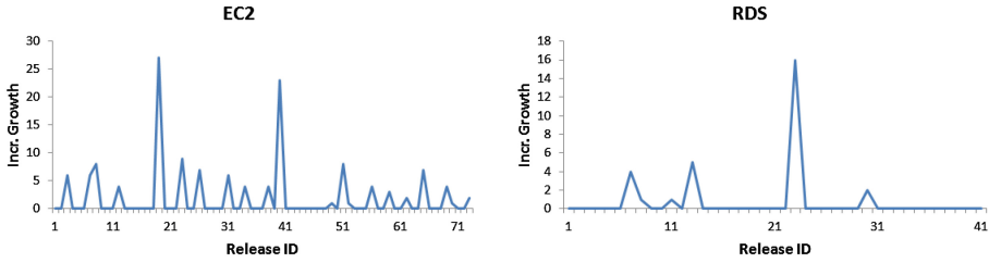
Fig. 3. Incremental growth—difference between the number of operations in subsequent service releases— per release ID.
