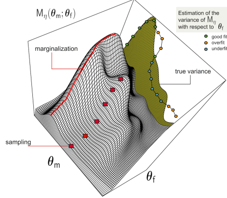
Fig. 2. For any pair of \theta_m and \theta_f we can compute the statistics for M , M_\eta(\theta_m; \theta_f) . Since we do regression over \theta_m , we model the relation between such values and \theta_f as the variance of a random variable, indexed by \theta_m , whose samples are the values, as a function of \theta_f . Marginalization is the exponential strategy that estimates such variance correctly; all downsampling strategies possibly over or under fitting. Accounting for the relation between this variance and \theta_m can be achieved by heteroschedastic regression.
