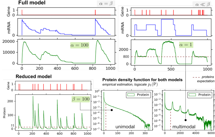
Fig. 5. Comparison between the dynamics of the full and the reduced models from §5.2, with k_{\text{off}} = k_{\text{on}} = \delta_P = 10^{-2} , \delta_{\text{RNA}} = 10 , [G_{\text{act}}]_0 = 1 . Values for transcription ( \alpha ) and translation ( \beta ) are reported in the figure. The reduced model predicts spiked dynamics, leading to a unimodal distribution of proteins. The larger model, instead, can either predict protein buffers, when there is no time scale separation ( \alpha = \beta ), or multiple equilibria, leading to a multimodal distribution of protein counts. Observe that the expectation on the number of proteins in the long run spans over different order of magnitudes, according to the relation between \alpha and \beta .
