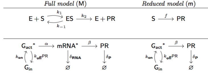
Fig. 3. Example models tested in this paper. Top panel: the Henri-Michaelis-Menten model, where \mathbf{m} is derived when \mathbf{C} : [\text{E}]_0 + [\text{ES}]_0 \ll [\text{S}]_0 + K_{\text{MM}} . Bottom panel, a protein translation network where \mathbf{m} when \mathbf{C} : \beta \gg \alpha .
