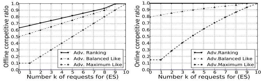
Fig. 1: (left) w.r.t optimal offline mechanism, (right) w.r.t. ADVISED RANKING
