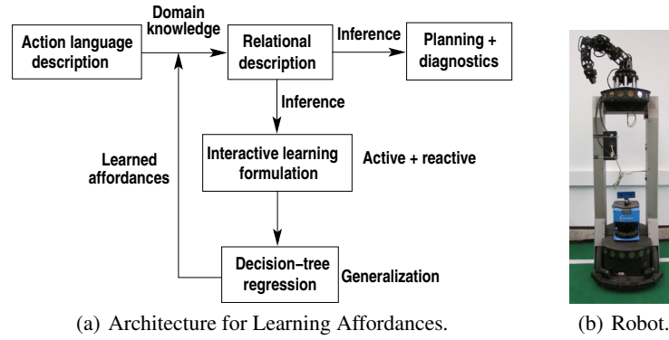
Fig. 1. Architecture combines non-monotonic logical reasoning and relational reinforcement learning for learning affordances.
