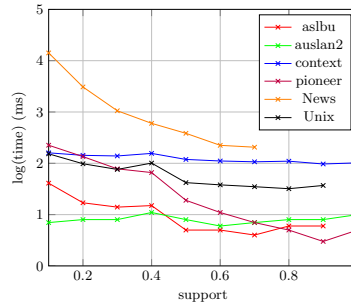
Fig. 5: Time needed to mine constraints.
