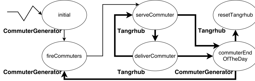
Fig. 5. Event Graph of the TRebeca Model
