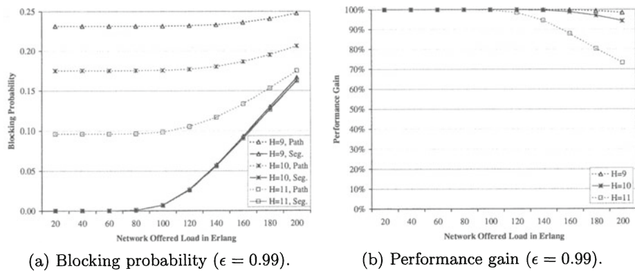
Fig. 8. Impact of H ( \epsilon = 0.99 ).
