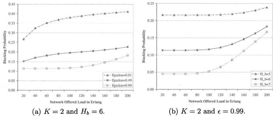
Fig. 2. Blocking probability of shared-path protection.
