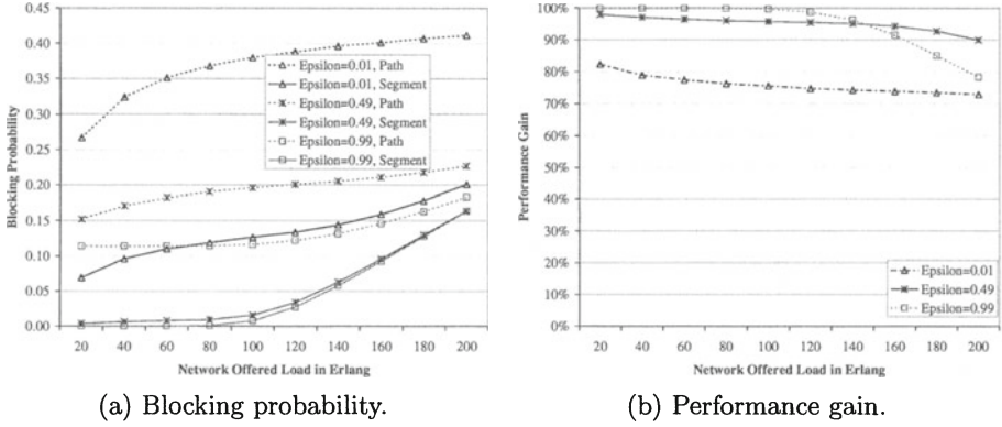
Fig. 5. Impact of \epsilon ( H_b = 6 ).
