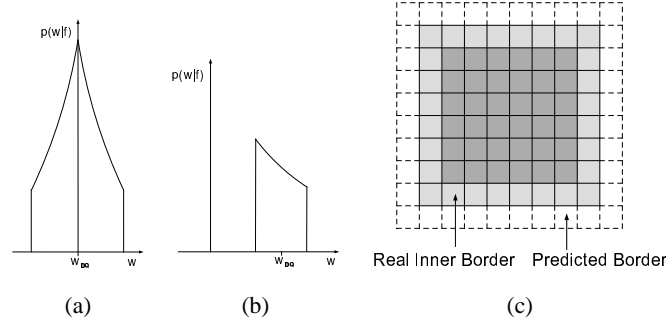
Fig. 1. Prior distribution of DCT coefficients given known quantised coefficients \mathbf{f} . (a) Zero-quantised coefficient. (b) Non-zero quantised coefficient. (c) Predicted border-pixels are given by inner border-pixels.
