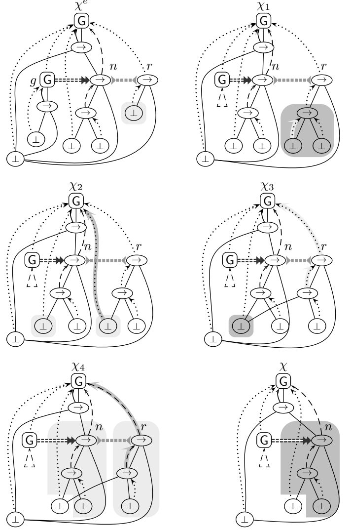
Figure 13: Example of solved instantiation edge
