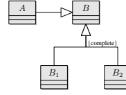
Fig. 5. Encoding of A \subseteq B_1 \sqcup B_2
