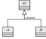
Fig. 4. Encoding of A \subseteq \neg B
