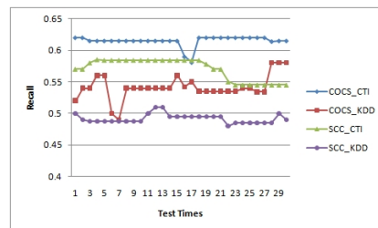
Fig. 3. Recall Comparison Results
