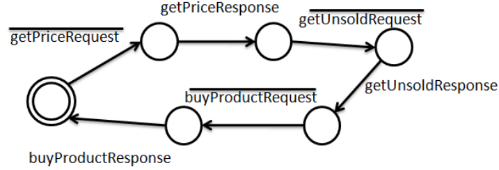
Fig. 13. LTS describing the behaviour of the IIOP vendor application
