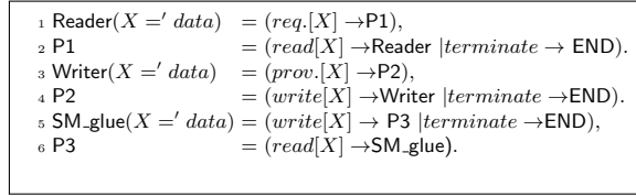
Fig. 22. Shared-memory middleware type specification
