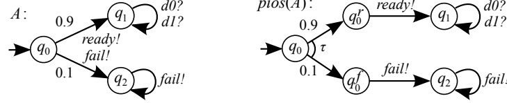
Fig. 2. Assumption A and its PIOS conversion \text{pios}(A) .
