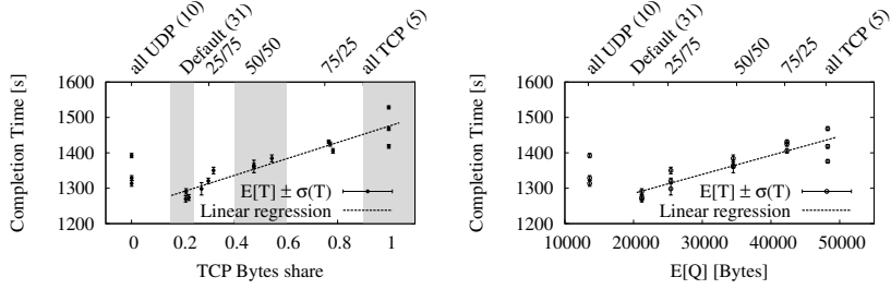
Fig. 4. Completion time as a function of the TCP vs uTP byte-wise share (left) and as a function of the average buffer size (right).
