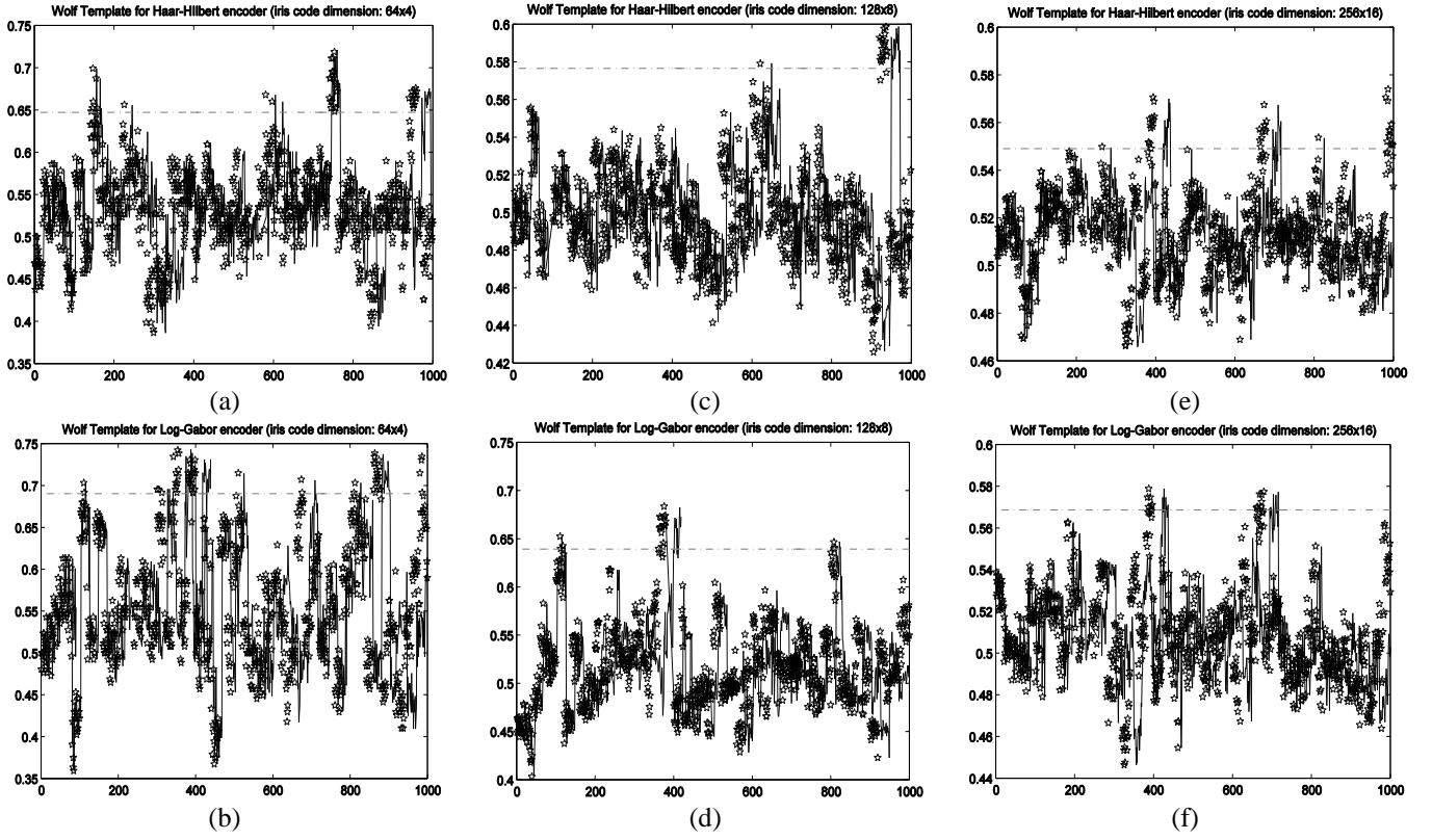
Fig. 3. The similarity scores corresponding to the impostor comparisons generated by the last wolf-templates obtained for Haar-Hilbert (64x4 – a, 128x8 – c, 256x16 – e) and Log-Gabor (64x4 – b, 128x8 – d, 256x16 – f) encoders.
