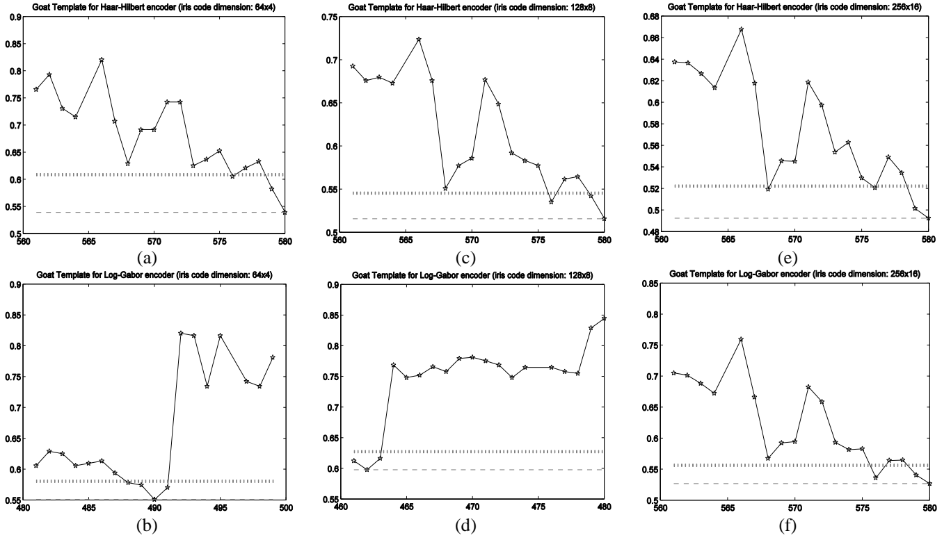
Fig. 2. The marginal goat-templates obtained for Haar-Hilbert (64x4 – a, 128x8 – c, 256x16 – e) and Log-Gabor (64x4 – b, 128x8 – d, 256x16 – f) encoders.
