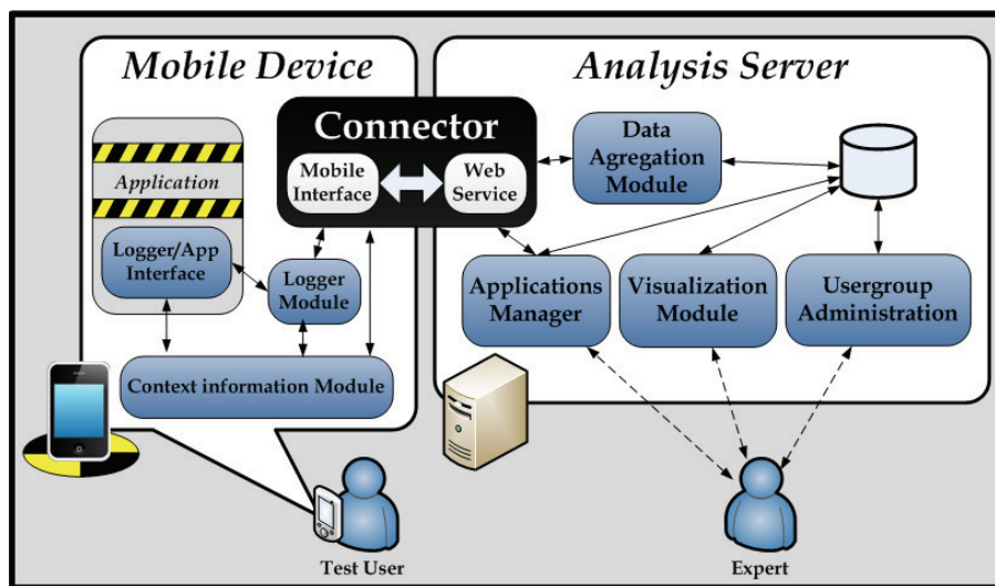
Fig. 2. System architecture
