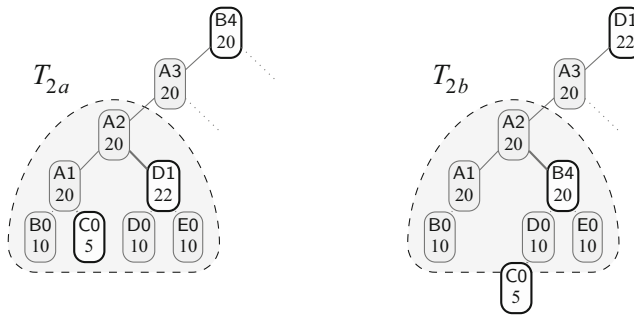
Fig. 2 Subtrees T_{2a} and T_{2b} for 9-key interval I_9 with h = 2 . T_{2a} is missing the two keys A3, B4; T_{2b} is missing A3, D1. Each node shows its equality key and the frequency of that key; split keys are not shown. (For each node, take the split key to be any key that separates the keys in the left and right subtrees.) The costs of T_{2a} and T_{2b} are 209 and 210, respectively, but in T_{2a} , the total weight of the keys is larger by 2
