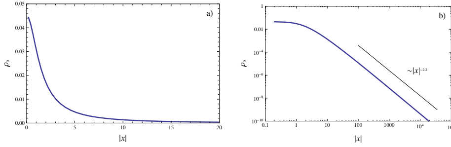
Fig. 1. The minimizer \rho_0 in Theorem 3.5 for a = 1 and b = 1 , plotted on a linear (a) and logarithmic (b) scale.
