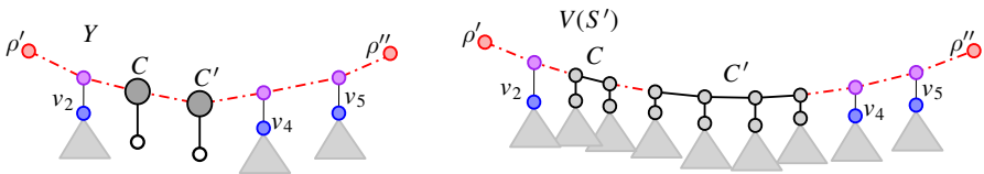
Fig. 8 The tree \mathcal{V}(S') achieved after the decomposition
