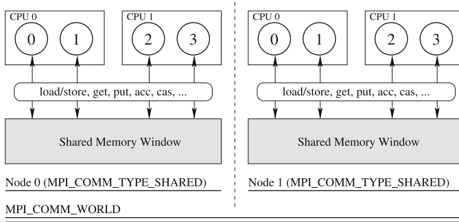
Fig. 1 Interprocess shared-memory extension using MPI RMA; an execution with two nodes is shown, and a shared memory window is allocated within each node. The circles represent MPI ranks running on two dual-core dual-socket nodes
