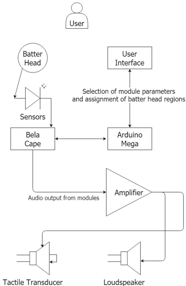
Fig. 1 Schematic of the DAD hardware system
