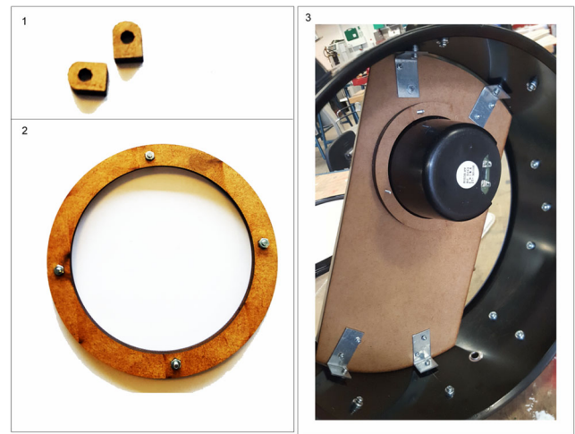
Fig. 2 Speaker Bracket System 1. Nut retainers 2. Laser Cut Bracket 3. Speaker Frame in Position Inside DAD
