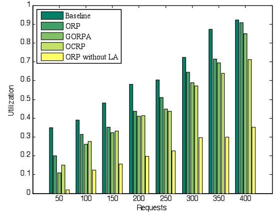
Fig. 8 Comparison between utilization of VMs
