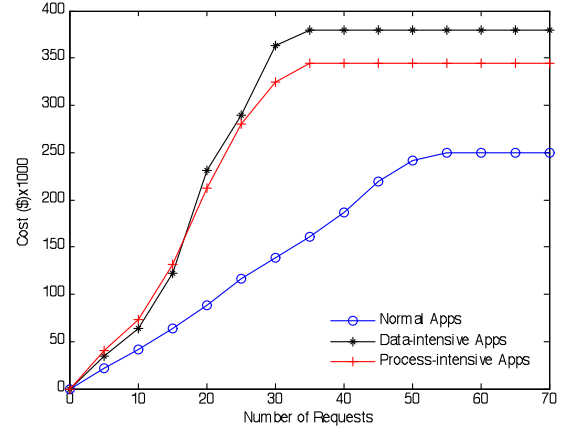
Fig. 10 Evolution of total costs in different types of demands with constant number of VMs
