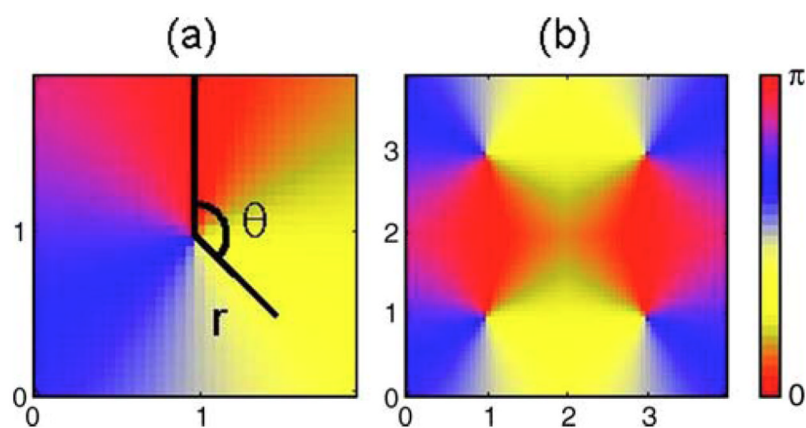
Fig. 5. Pinwheel architecture in the model. (a): a single pinwheel system. Each cell is indexed by its distance r from the pinwheel center at (1,1) , and an angle \theta measured relative to the depicted vertical line. The preferred orientation of the cell is \theta/2 . (b): four pinwheel system, with centers at (1,1) , (1,3) , (3,1) , and (3,3) . \theta of each cell is defined relative to the nearest center. The red regions show the two horizontal columns – each connecting center pairs with opposite parity
