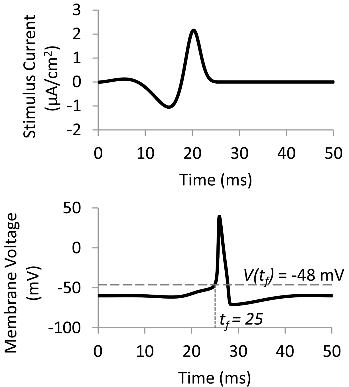
Fig. 3. The optimal stimulus derived from the gradient algorithm (top) triggers a single action potential in the Hodgkin-Huxley model (bottom)
