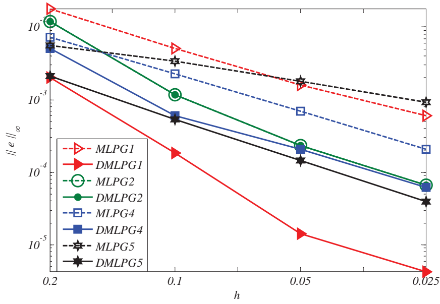
Fig. 1 Comparison of MLPG and DMLPG methods in terms of maximum errors.
