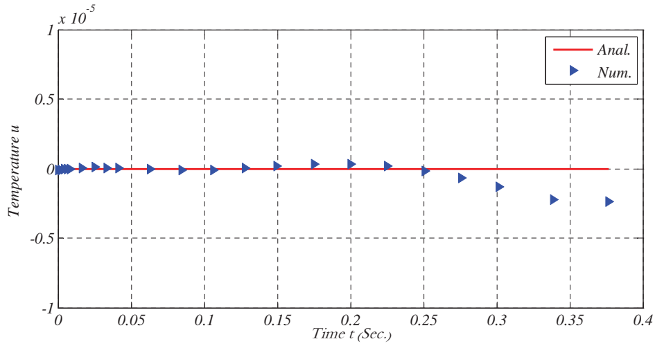
Fig. 3 Accuracy of method for early time instants at position x_1/a = 0.5 .
