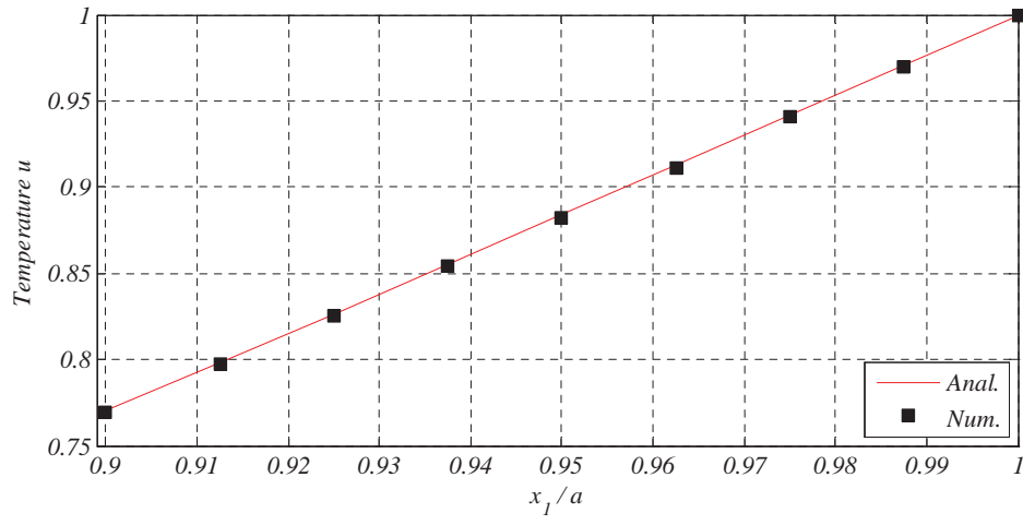
Fig. 4 Accuracy of method for points close to the thermal shock at time t(70) sec.
